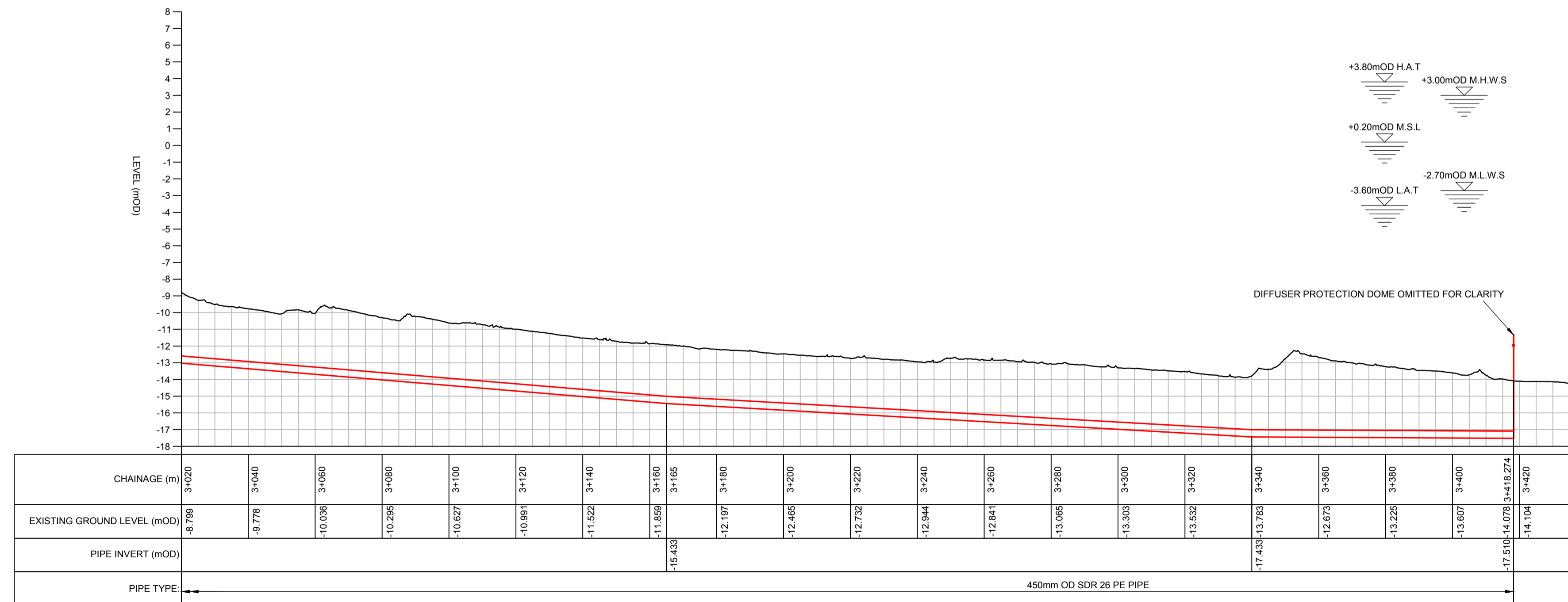
LONGITUDINAL SECTION THROUGH LONG SEA OUTFALL - MARINE SECTION SCALE: H-1:1000 / V-1:200
